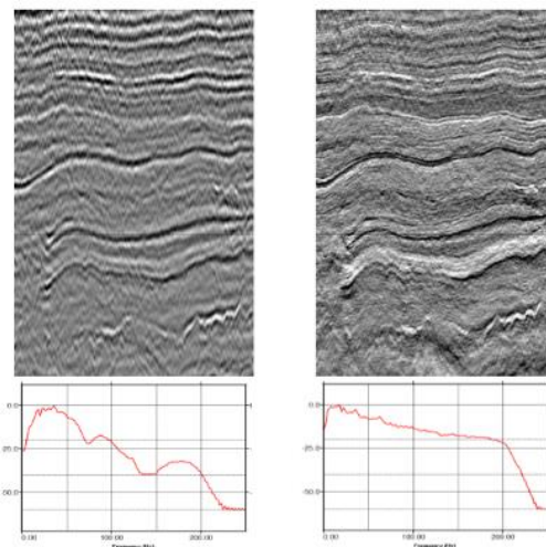
Figure 4: Comparison of images (top), amplitude spectra (bottom) acquired with: flat streamer and conventional source (left) and variable depth streamer and synchronized multi-level source (right). Data courtesy of Lundin
