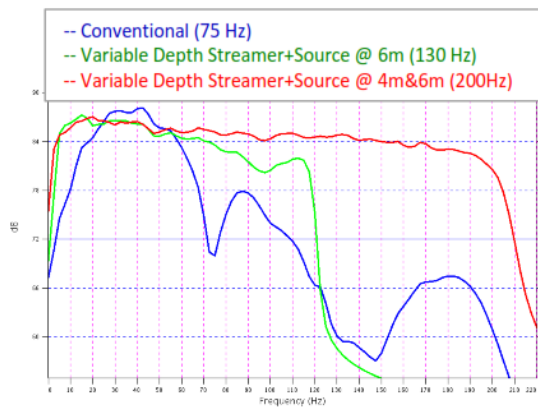
Figure 3: Comparative amplitude spectra of seismic images obtained with different type of acquisition. The combination of a variable depth streamer with a synchronized multi-level source allows a 7 octave-image-bandwidth.
