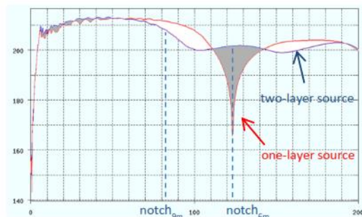
Figure 2. Amplitude spectra gain of synchronized two-level source array with airguns at 6 m and 9 m.
