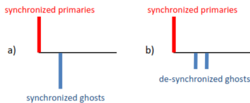
Figure 1: Primaries and ghosts of two synchronized airguns a) airguns at same depth b) airguns at two different depths
