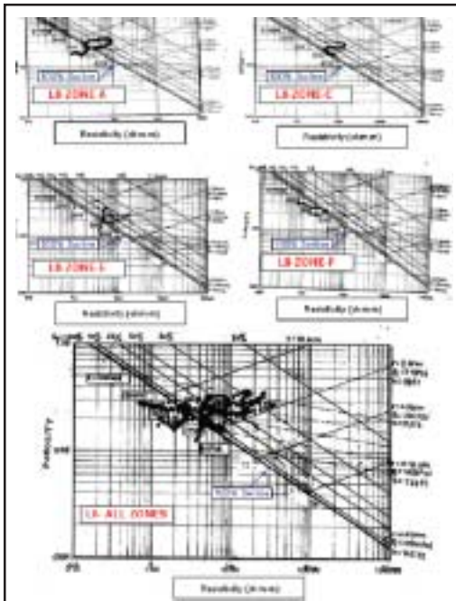
Fig. 8: Pickett plot for LII -Zone-A, Zone-C, Zone-E and All Zones
