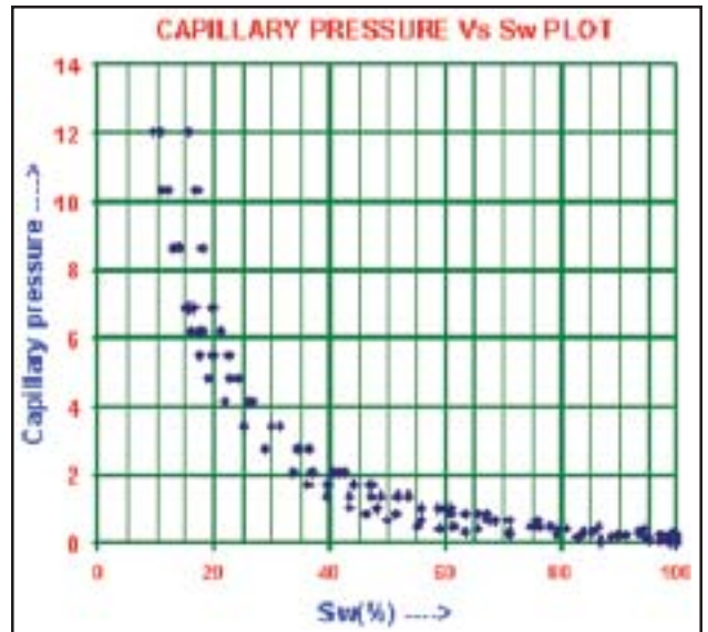
Fig. 5: Capillary pressure Vs Sw plot (core data).
