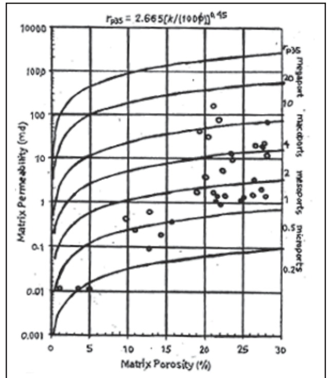
Fig. 4: Aguilera equation for pore throat aperture
