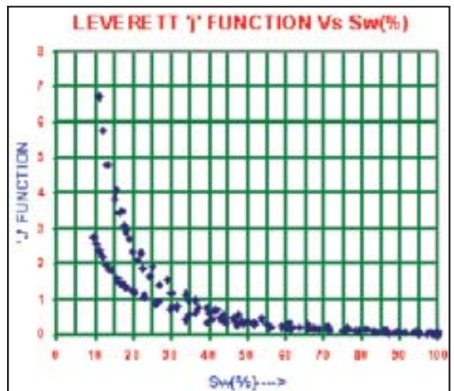
Fig. 6: Leverett ‘J’ function Vs Sw plot (core data).
