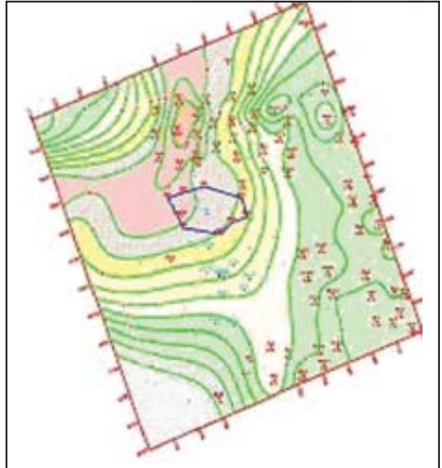
Fig.6 : Well based net pay thickness map
