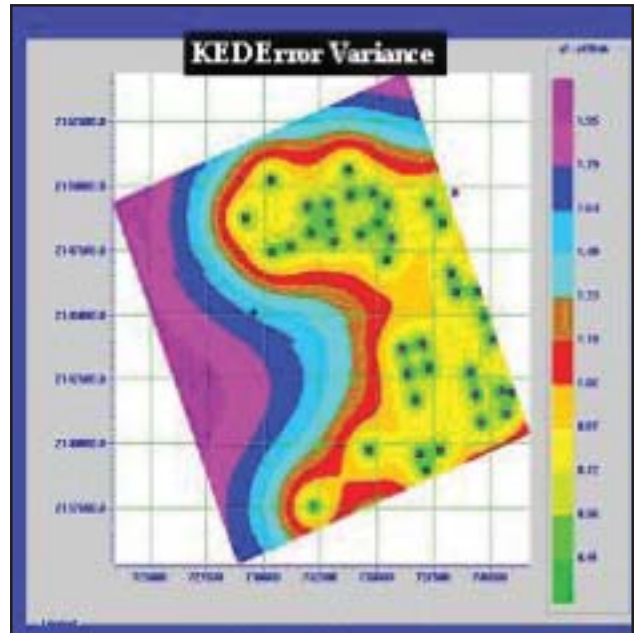
Fig.13 : Error variance after performing KED operation.
