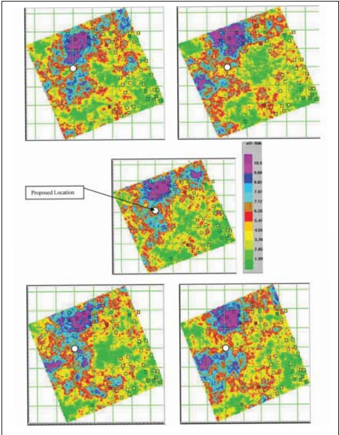
Fig.9 : 5 conditional simulation maps out of 25 realizations showing variation of effective thickness in interval space but honouring the well data everytime.
