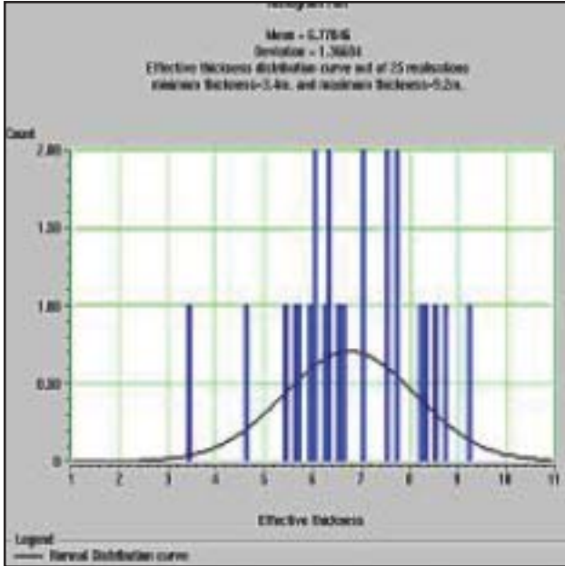
Fig.10: Histogram with normal distribution curve showing thickness sampled at proposed location out of 25 simulated maps
