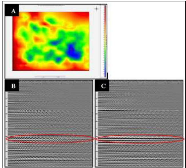
Fig. 9: A) example map of the velocity difference for Sb horizon before and after full azimuth anisotropic tomography, B) "spiral gather" before and C) after full azimuth anisotropic tomography and migration.
