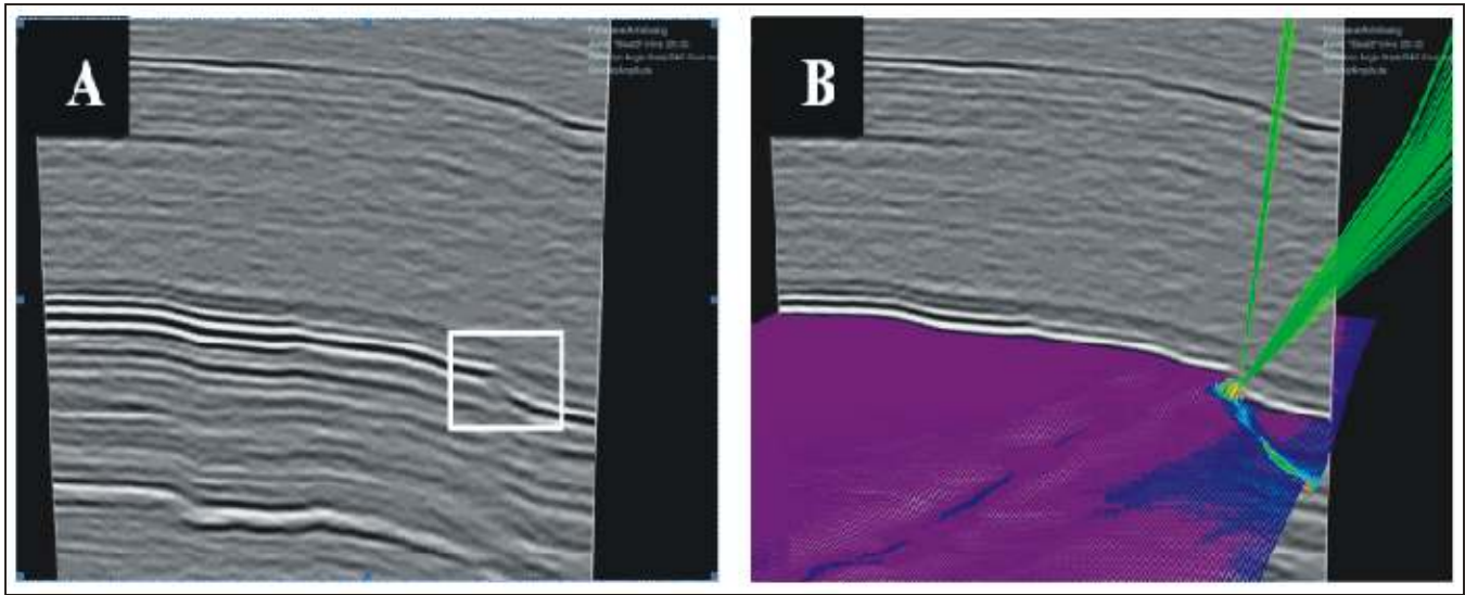
Fig. 16: Analysis of target illumination. A) the place of poorer illumination, B) map of illumination (weak - red, yellow, blue, strong - purple) and rays connected with actual geometry
