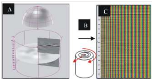
Fig. 8: A) 3D cylindrical spiral CRP gather reflections as a function of depth azimuth and reflection angle. Presented are traces for given azimuth, and for all angles, B) the idea how 3D CRP gather is unwrapped into 2D plane, C) unwrapped "spiral" gather 2000 traces. Color presents periodical change of azimuths.
