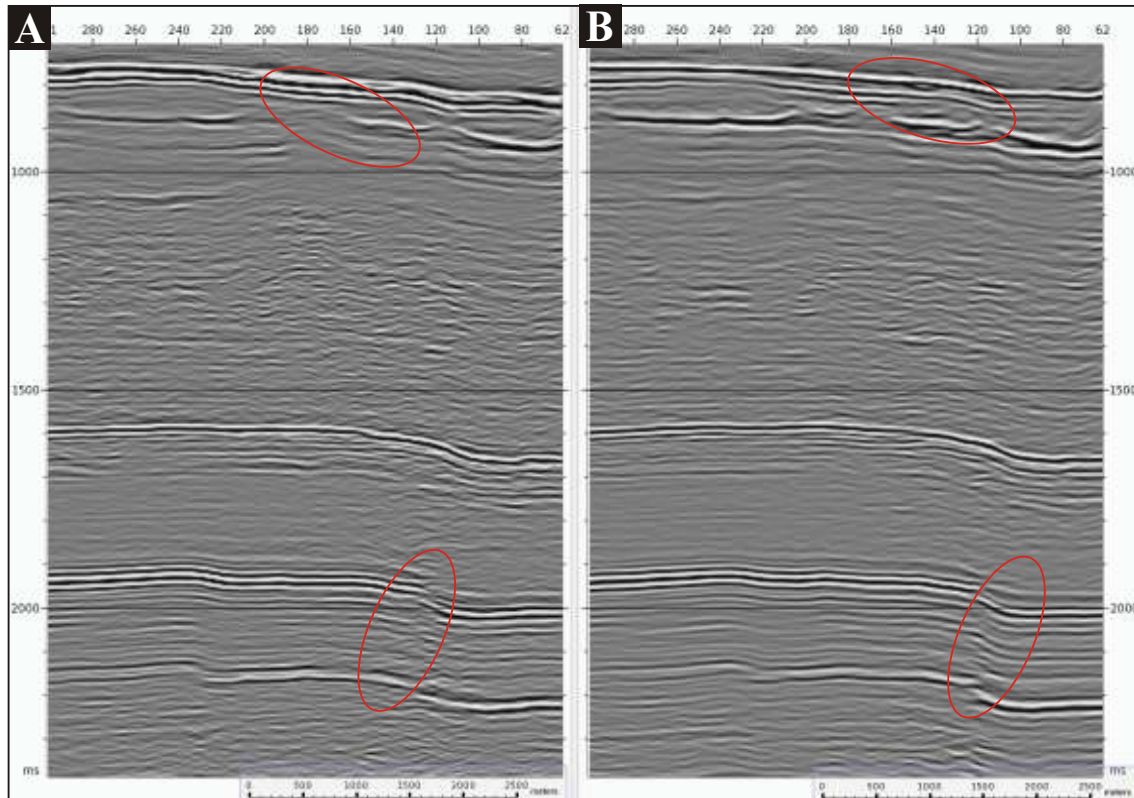
Fig. 15: Results of A) PreSTM and B) PreSDM.
