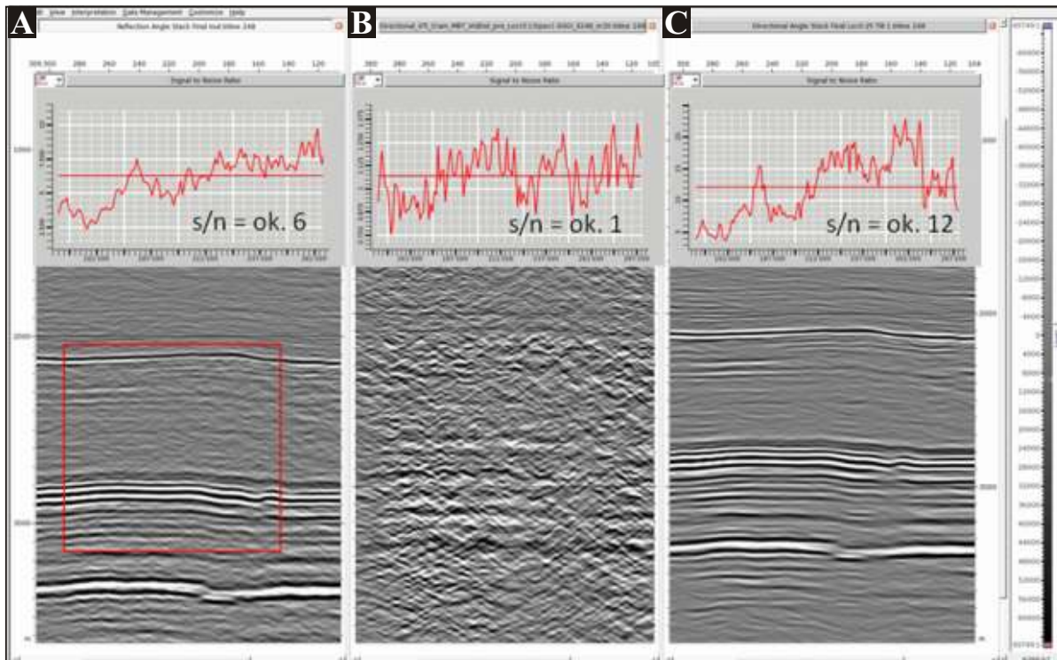
Fig. 13: A) original directional stack, B) diffraction stack, C) specular stack. The s/n (signal to noise) ratio is shown for each stack. The stacks were created from gathers presented on Fig.12.
