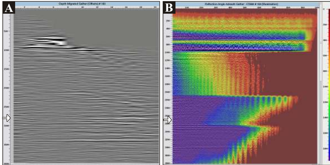
Fig. 14: Relative amplitudes reconstruction. A) Kirchhoff PreSDM CRP gather, B) full azimuth angle domain migration CRP gather (colors show illumination of the gather).
