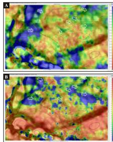
Fig. 10: Maps of effective parameters of azimuthal anisotropy for Or horizon. A) based on RMOs, B) based on amplitudes. Intensity is shown in colors (blue higher intensity) and length of black dashes. Azimuth of fractures' strike (direction of fast velocity) is shown as orientation of dashes. White arrows are drawn on the maps in the places of higher intensity (the same places) to compare azimuths.
