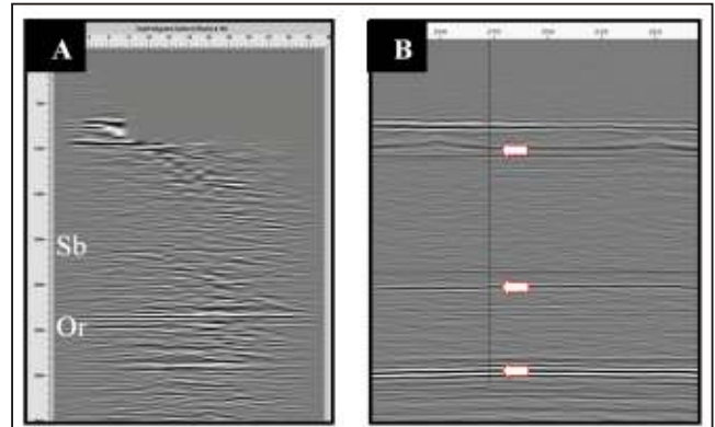
Fig. 5: Results of final (stage 1) isotropic Kirchhoff PreSDM. A) CRP gather, B) stack.
