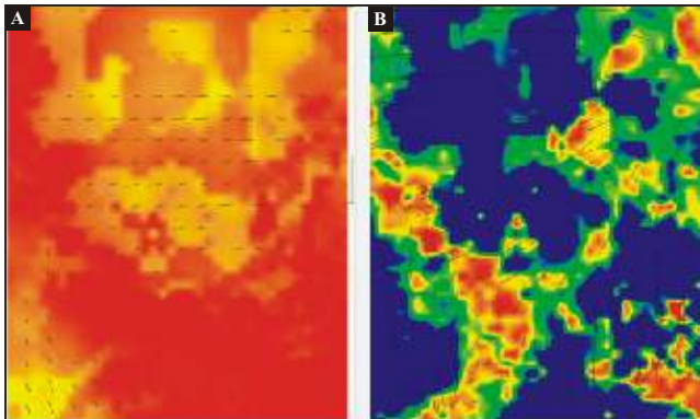
Fig. 11: Maps of parameters of azimuthal anisotropy for Sb-Or layer calculated based on kinematic attribute. A) effective parameters, B) parameters for bottom of the layer. Intensity is shown in colors (blue higher intensity) and length of black dashes - the same scale for both. Azimuth of fractures' strike (direction of fast velocity) is shown as orientation of dashes.
