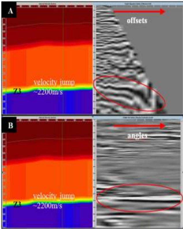
Fig. 3: Comparison of signal stretching by A) 3D Kirchhoff offset domain PreSDM and B) 3D CRAM - common reflection angle domain pre-stack depth migration.
