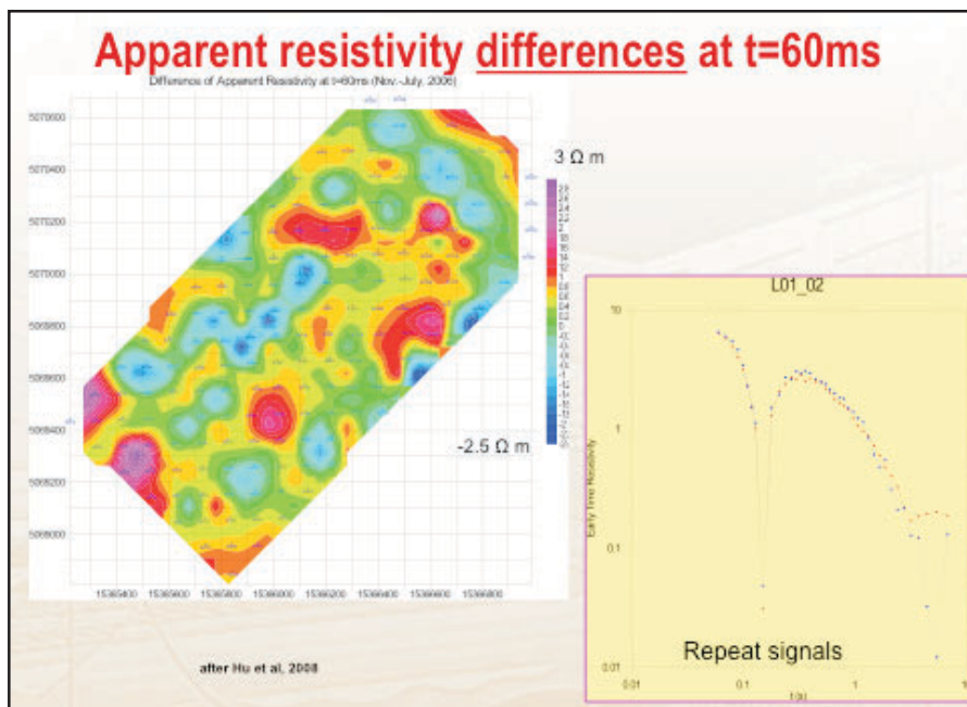
Fig.3 Time lapse difference map (apparent resistivities) from the steam flood example from China. On the right are two individual signals from the same location.
