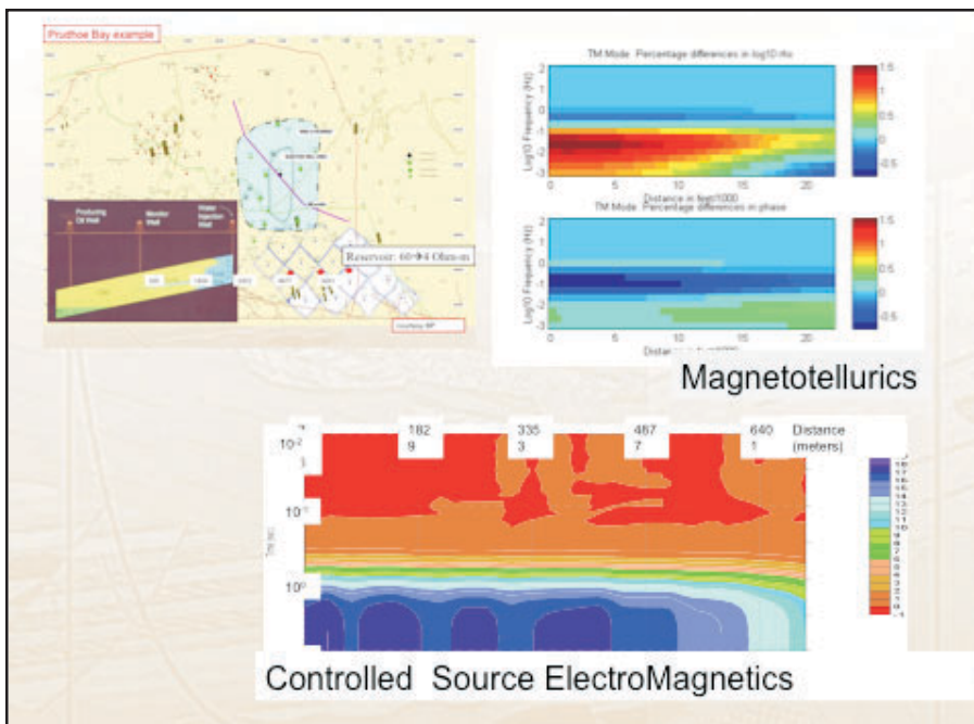
Fig.2 Results from the feasibility study for Prudhoe Bay, Alaska. On the top left is the survey map with the seismic profile that yielded the a priori information. The insert in the map is the reservoir model cartoon. On the right and the bottom are the time-lapse results from EM monitoring numerical experiments.
