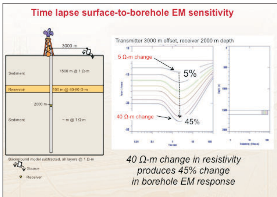
Fig.4 Feasibility models and results for surface-to-borehole EM monitoring. On the left is the model and on the right of the diagram the various curves for different reservoir fluid saturations.
