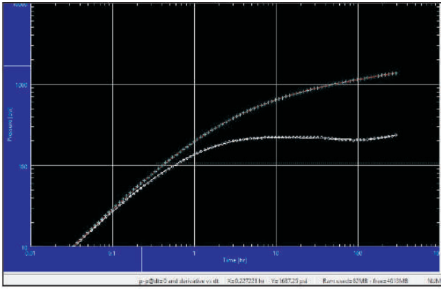
Fig. 1: Log Log de-convolution Plot with time for Well X-4
