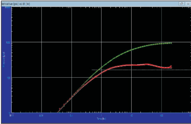
Fig. 3: Log Log Plot with time for Well X-4
