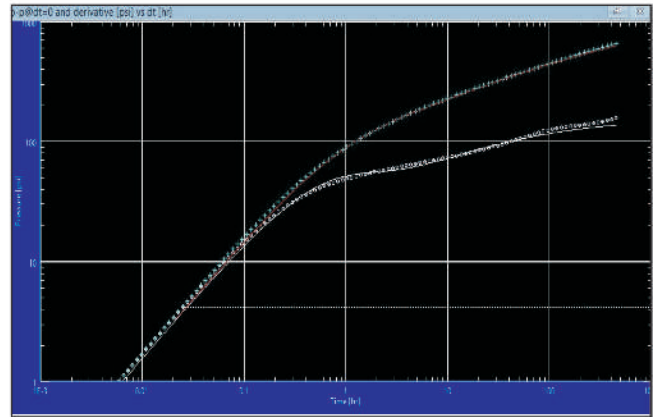
Fig. 5: Log Log de-convolution Plot with time for Well X-3
