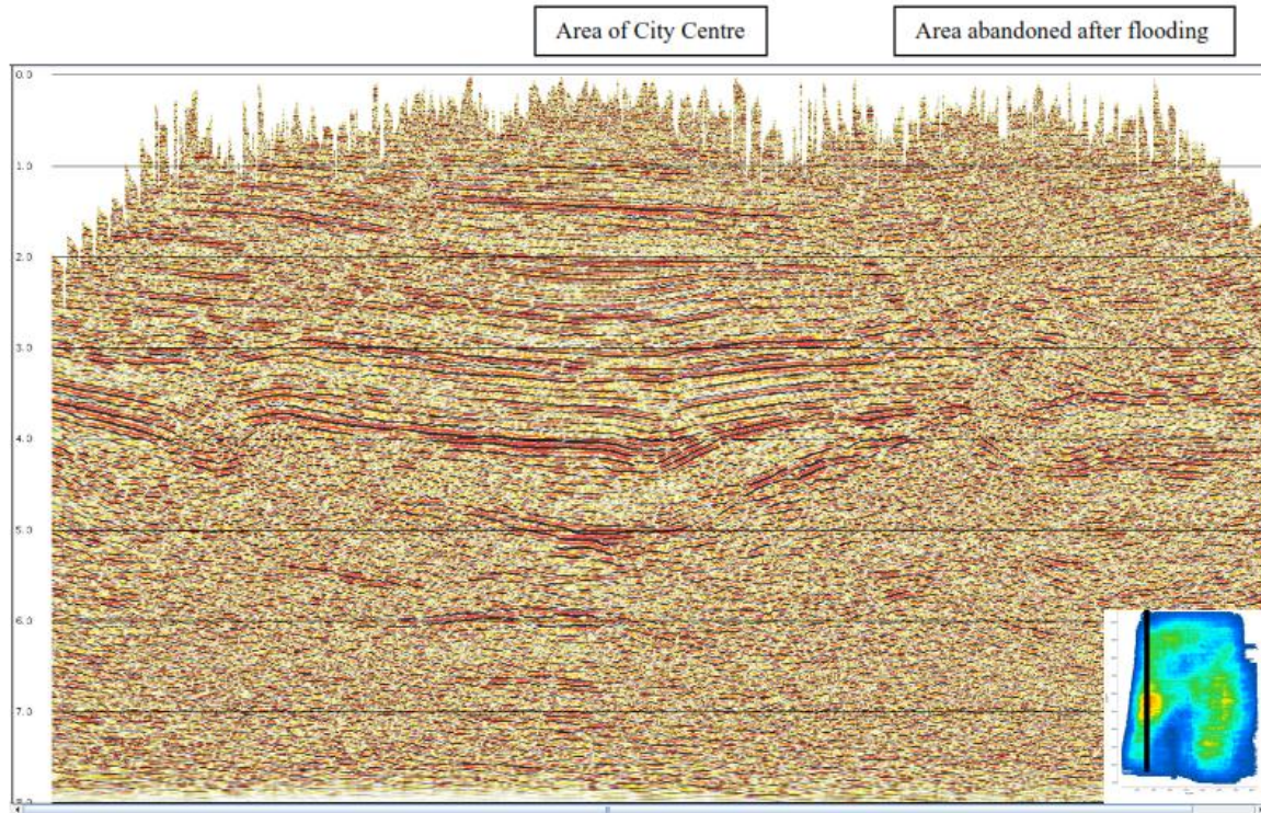
Figure 4: Post-stack QC migration of crossline from the survey. The black line on the inset fold map shows the line location, with the warm colours indicating the higher fold in the centre of the city. The degradation of the data quality on the right corresponds with the lower fold caused by the abandonment of that portion of the survey after the flooding. This is indicated by the blue colours in the South central part of the fold map.
